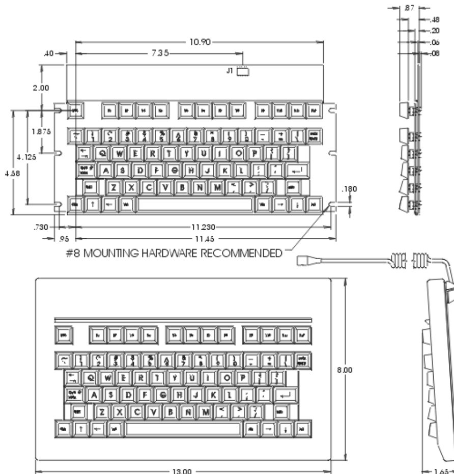
3075 ASCII, XT/AT Keyboard
